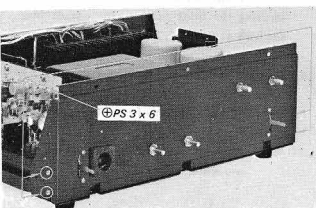
Fig. 2-4 Front subchassis removal
